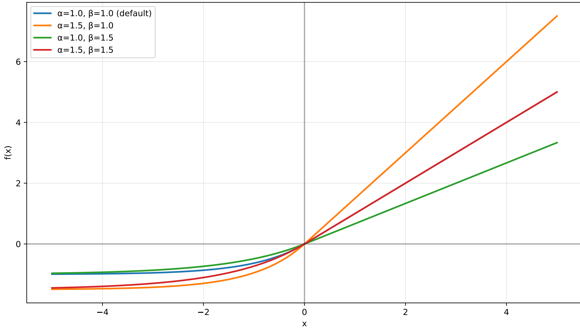
PELU Activation Function with Different Parameters
