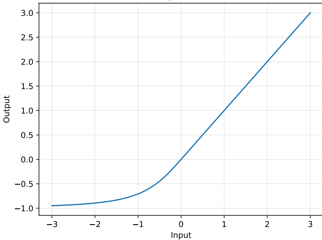
ISRLU (Inverse Square Root Linear Unit)
