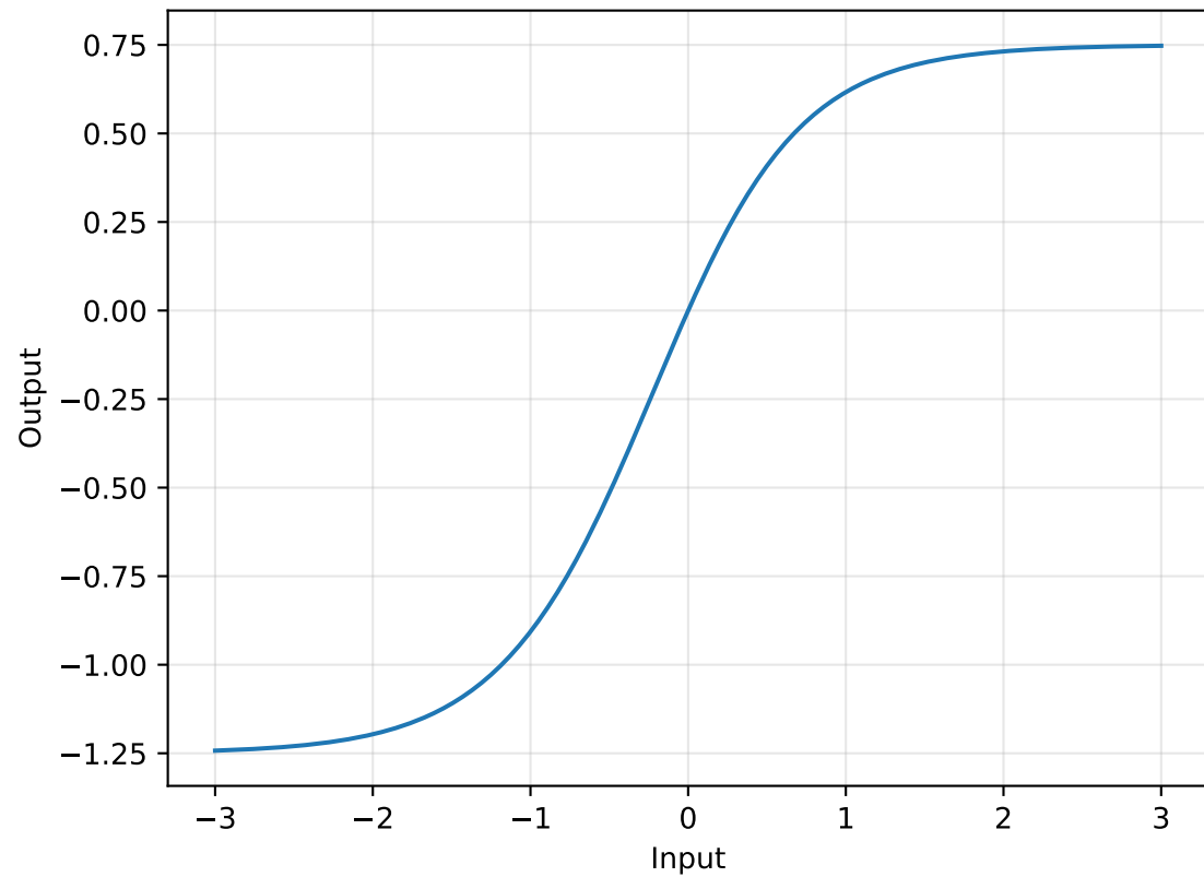
Penalized Tanh
